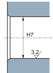
Mating Housing
